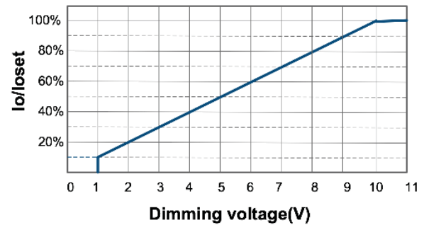
Io/Ioset vs. Dimming voltage
